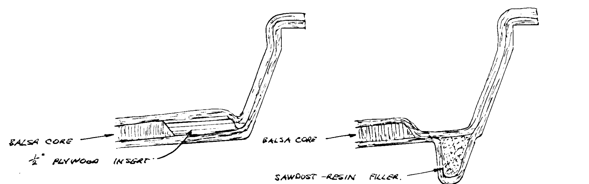
SECTION THROUGH STANTION BASE AREA SECTION THROUGH TOERNAL AREA.
